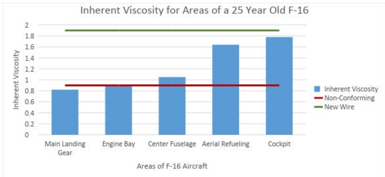
Figure 3 Inherent Viscosity for Areas of a 25-Year-Old F-16
